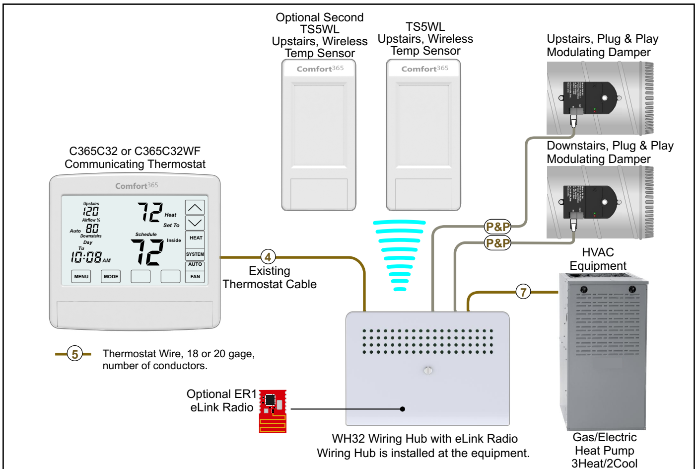
Wireless installation for replacement installation.
