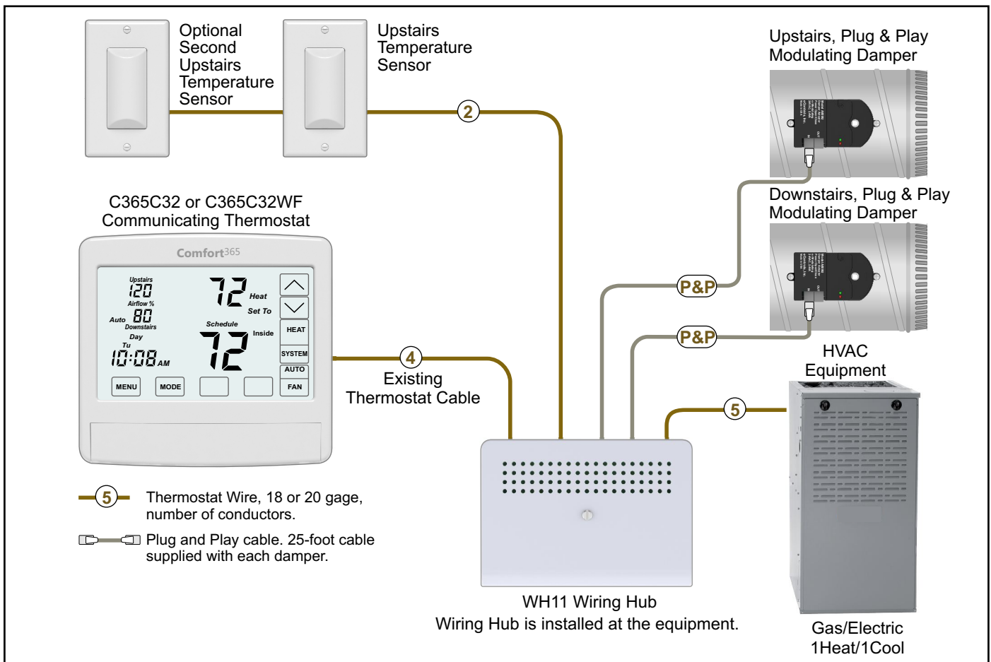
Wired installation for RNC.
